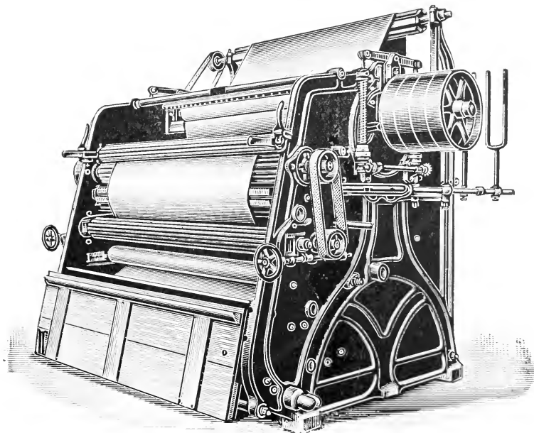
FIG. 35.—Cloth-washing Machine.
